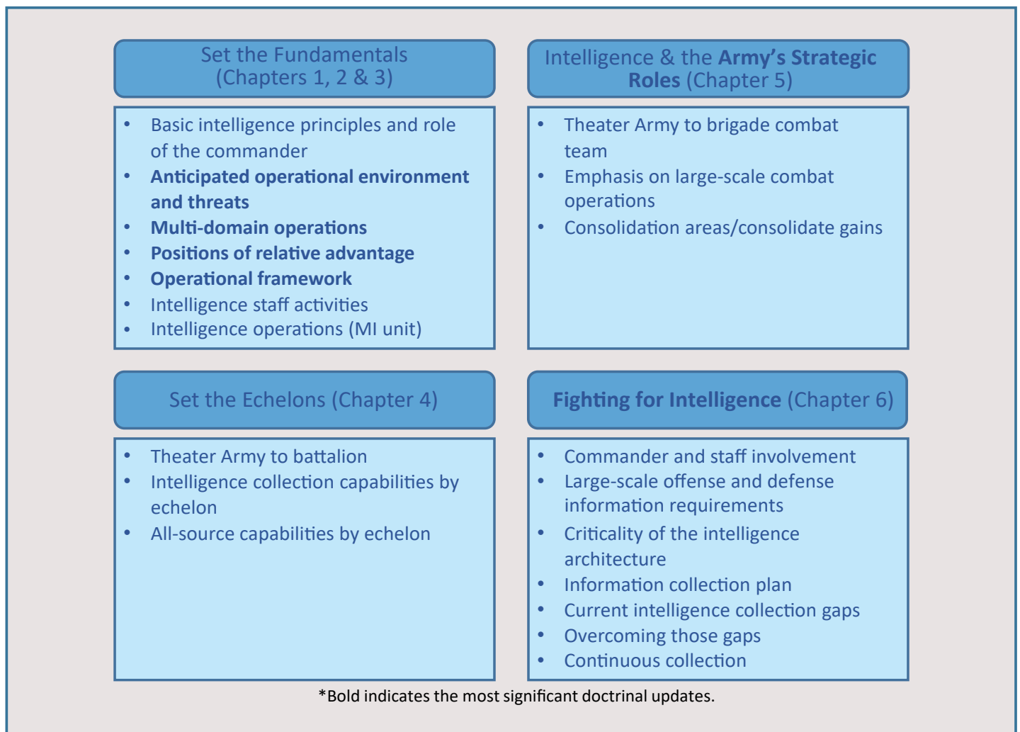
Figure 2. FM 2-0 Structure
