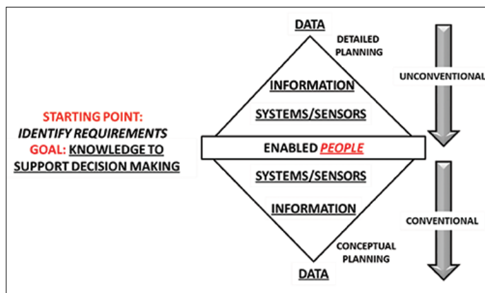
Figure 2. Data-First Approach
